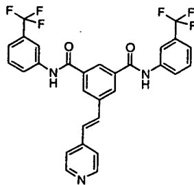
Compound # 16
